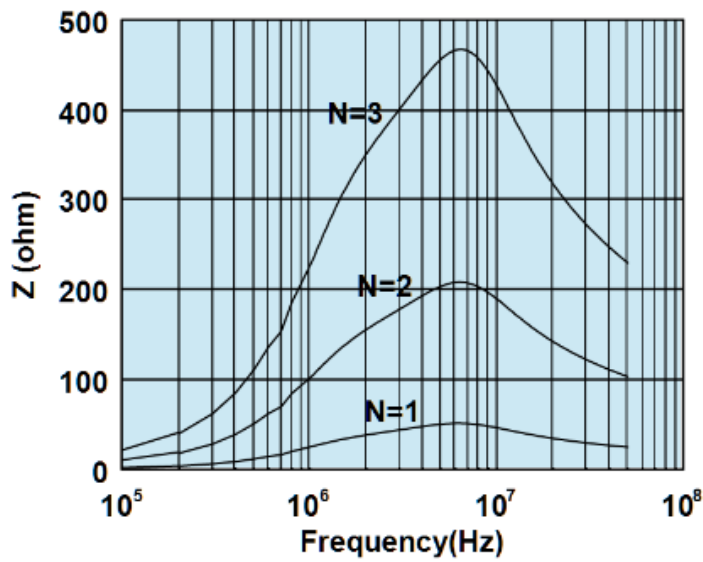
Impedance vs. frequency with one, two, and three turns.
